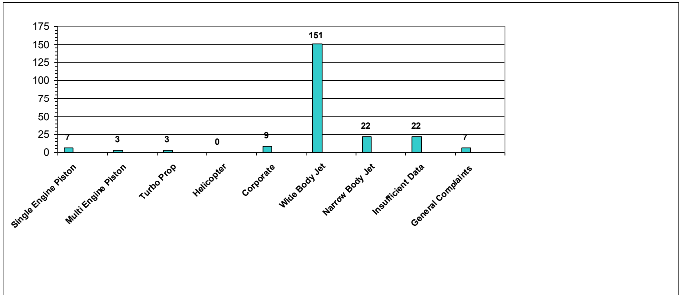
Figure C (1): Summary of Second Quarter 2013 Noise Calls for Civil Aircraft Operations by Aircraft Type
