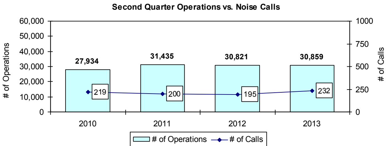
Figure A: Correlation between flight operations and flight related noise calls Second Quarter 2010-2013.
