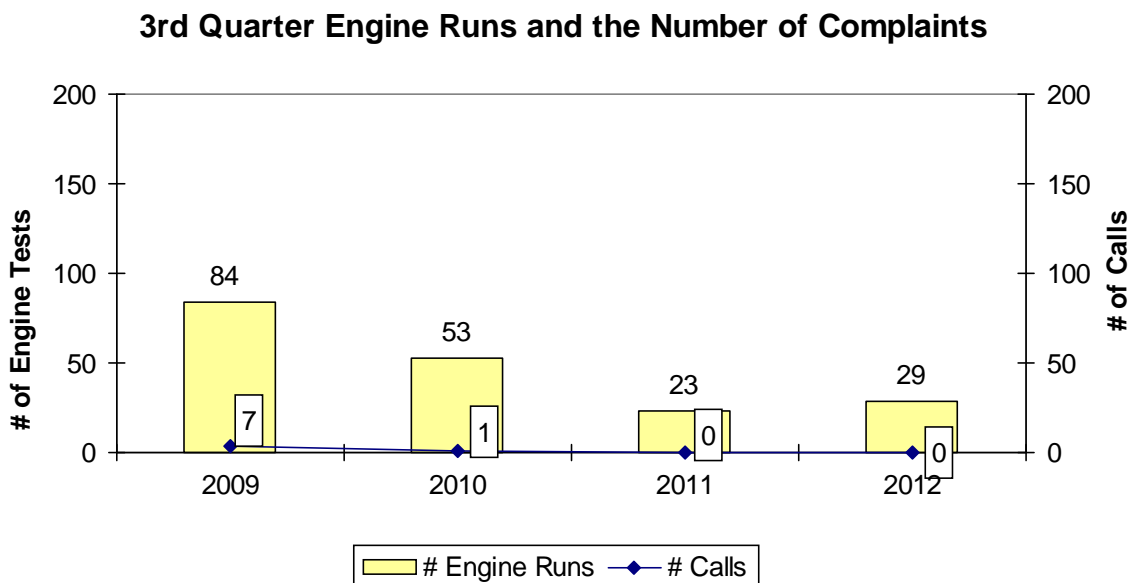
Figure B: Correlation between engine testing and engine testing related noise calls Third Quarter 2009-2012.
